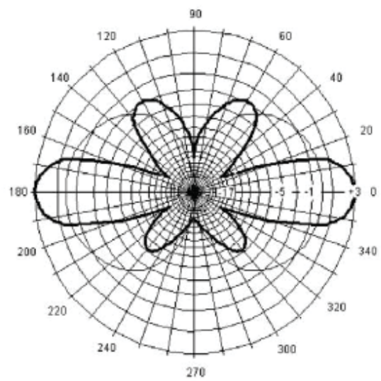
MFB1503 Elevation Pattern
