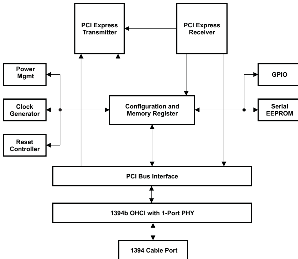
Figure 3-1. XIO2221 Block Diagram
