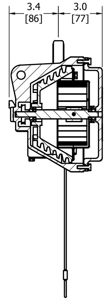
SECTION B-B
