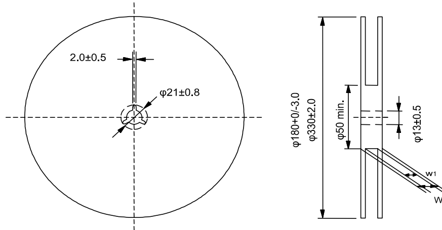
Fig.3 Taping Diagram
