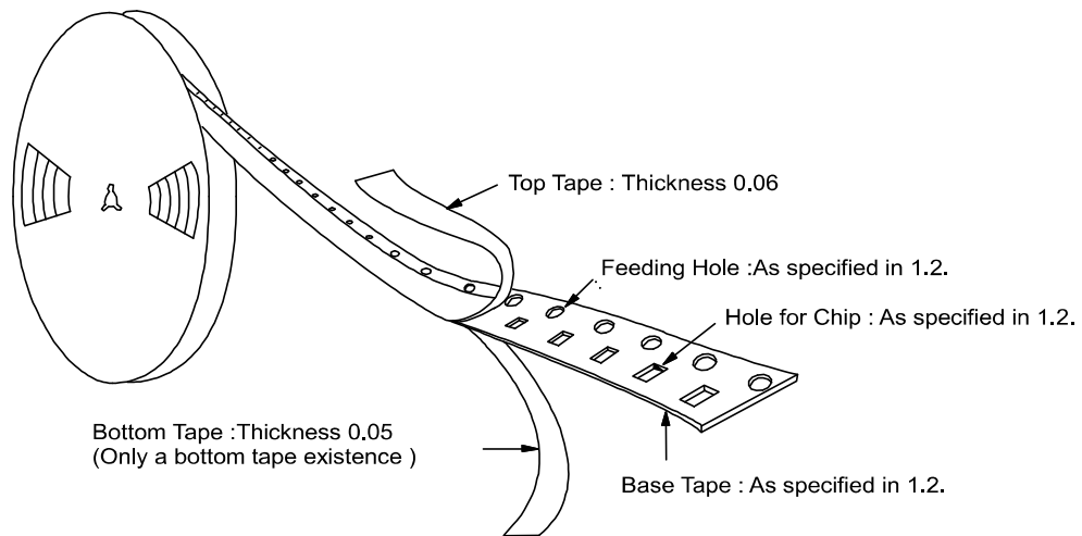
Fig.3 Taping Diagram
