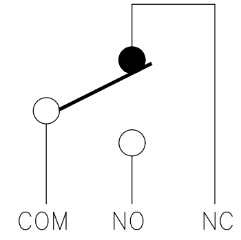
CIRCUIT DIAGRAM
