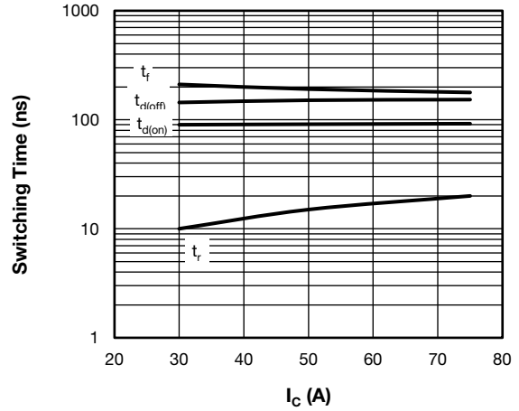
Fig. 8 - Typical Trench IGBT Switching Time vs. I_C (with Antiparallel Diode) T_J = 125^\circ C , V_{CC} = 600 V , R_g = 4.7 \Omega , V_{GE} = +15V/-15V , L = 500 \mu H
