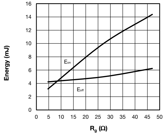
Fig. 9 - Typical Trench IGBT Energy Loss vs. R_g (with Antiparallel Diode) T_J = 125^\circ C , V_{CC} = 600 V , I_C = 75 A , V_{GE} = +15V/-15V , L = 500 \mu H
