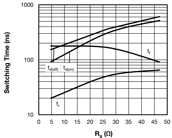
Fig. 10 - Typical Trench IGBT Switching Time vs. R_g (with Antiparallel Diode) T_J = 125^\circ C , V_{CC} = 600 V , I_C = 75 A , V_{GE} = +15V/-15V , L = 500 \mu H
