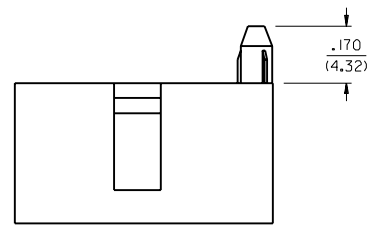
VIEW OF HOUSING SHOWING OPTIONAL LOCKING PEG
