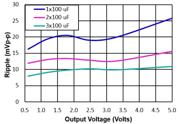
Figure 38. Output ripple voltage for various output voltages with external 1x100µF, 2x100µF, and 3x100µF ceramic capacitors at the output (3A load). Input voltage is 12V.
