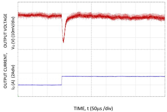
Figure 16. Transient Response to Dynamic Load Change from 50% to 100% at 12Vin, Cout-4x100µF, Ctune-4.7nF, Rtune-400
