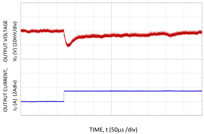
Figure 4. Transient Response to Dynamic Load Change from 50% to 100% at 12Vin, C out -2x330µF, 6x100µF, C tune -10nF, R tune -500
