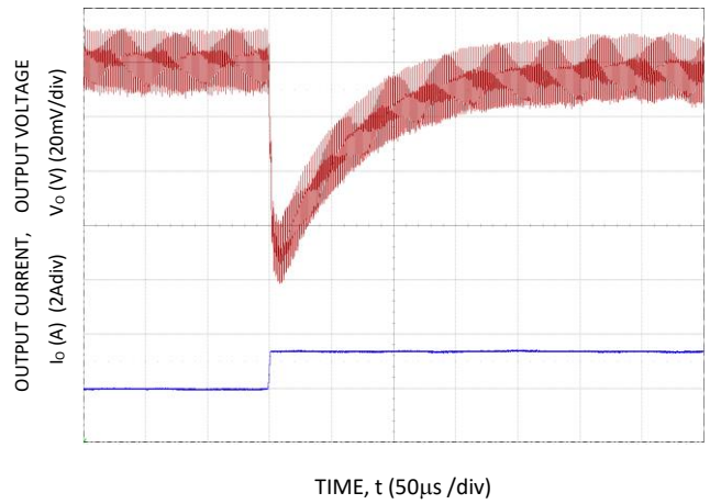
Figure 34. Transient Response to Dynamic Load Change from 50% to 100% at 12Vin, Cout-1x100µF, Ctune-680pF, Rtune-500
