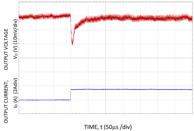
Figure 10. Transient Response to Dynamic Load Change from 50% to 100% at 12Vin, C_{out}=4\times 100\mu\text{F} , C_{tune}=4.7\text{nF} , R_{tune}=400
