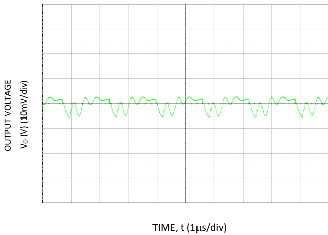
Figure 15. Typical output ripple and noise (Co=88µF ceramic, VIN = 12V, Io = Io,max.).
