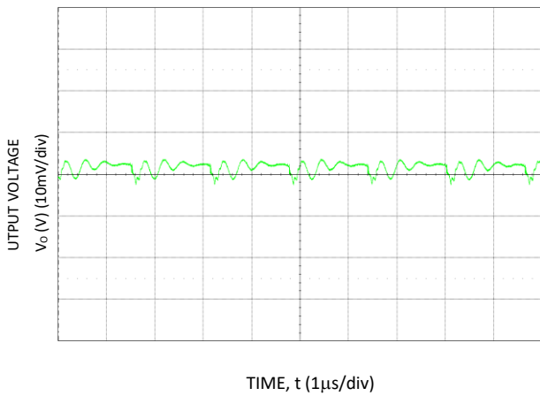
Figure 3. Typical output ripple and noise (C o =88µF ceramic, V IN = 12V, I o = I o,max ).
