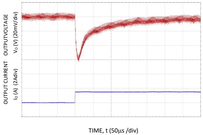
Figure 28. Transient Response to Dynamic Load Change from 50% to 100% at 12Vin, Cout=2x100µF, Ctune=1nF, Rtune=500
