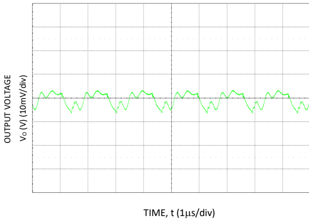
Figure 21. Typical output ripple and noise (Co=88μF ceramic, Vin = 12V, Io = Io,max.).
