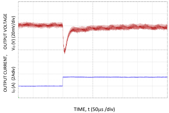
Figure 22. Transient Response to Dynamic Load Change from 50% to 100% at 12Vin, Cout-2x100μF, Ctune-1.5nF, Rtune-500
