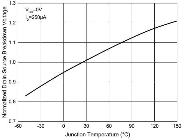
Fig. 7 - Normalized Drain-Source Breakdown Voltage
