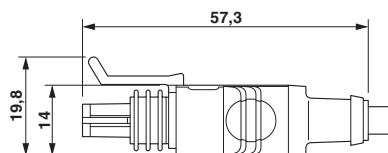
Dimensional drawing
