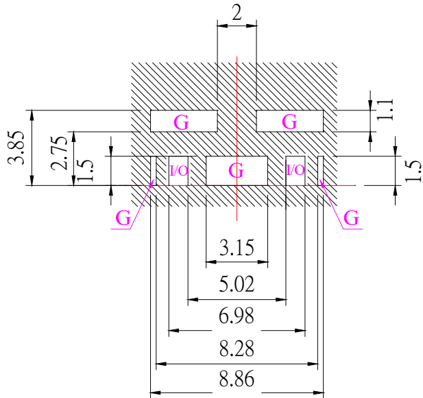
3-2-2 Solder resist Patten
