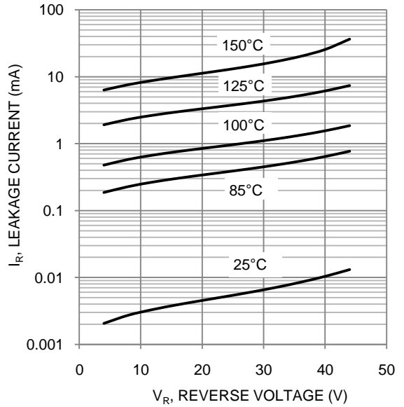
Figure 2. Typical Reverse Characteristics
