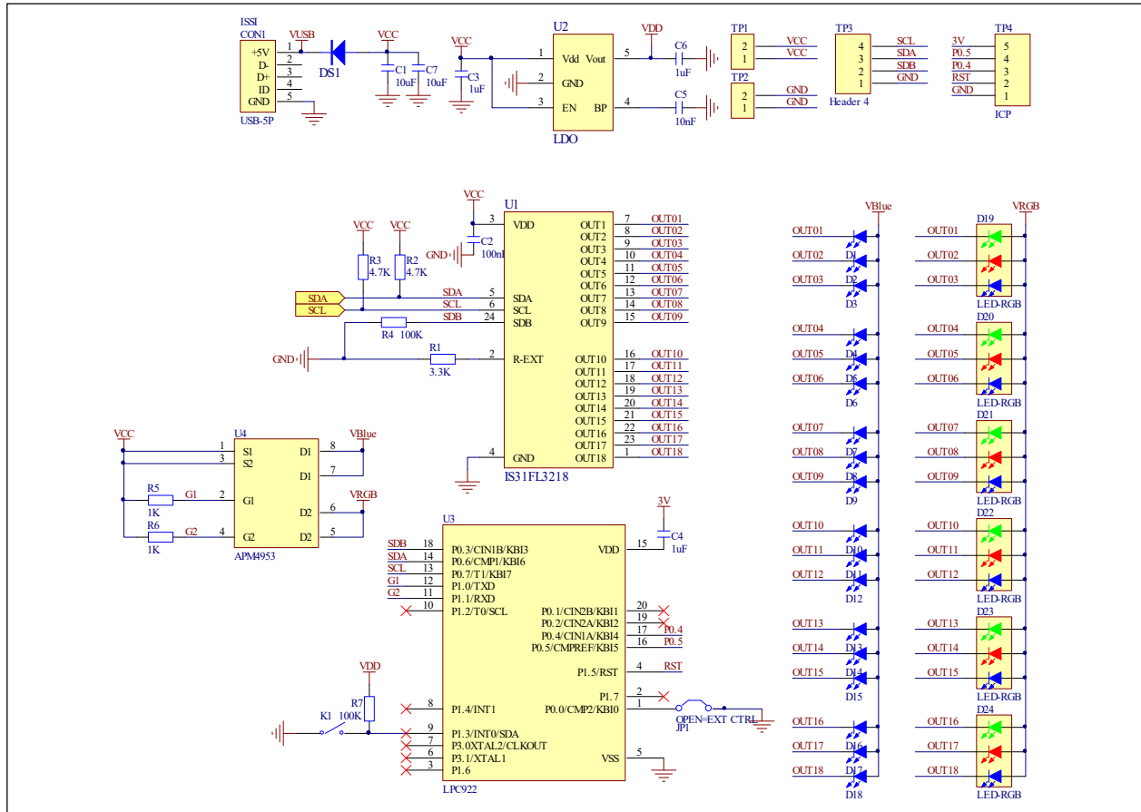
Figure 3: IS31FL3218 Application Schematic
