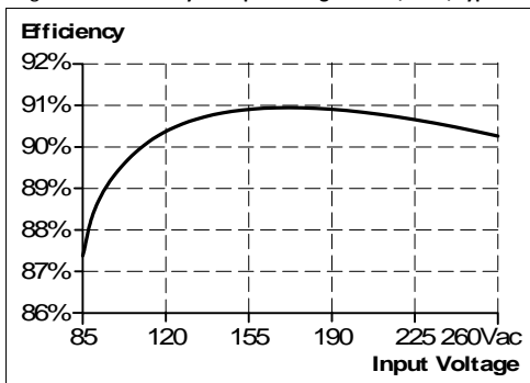
Fig. 8-3 Efficiency vs. input voltage at 24V, 1.5A, typ.
