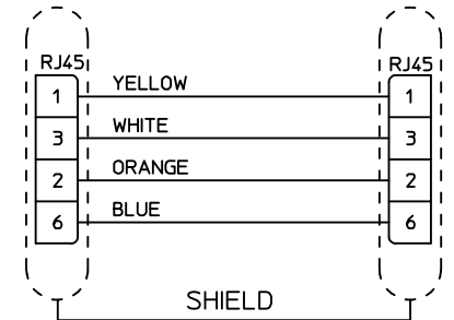
WIRING DIAGRAM
