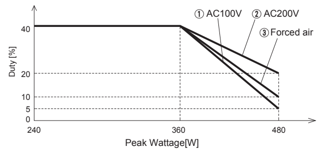
Fig.6.1 Derating of peak loading
