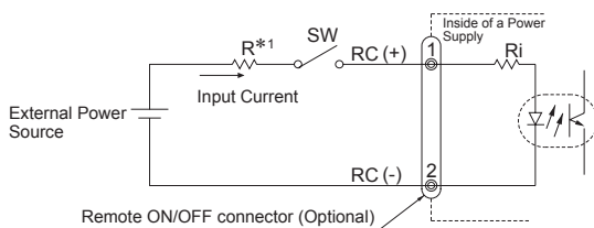
Fig.6.2 Example of using a remote ON/OFF circuit
