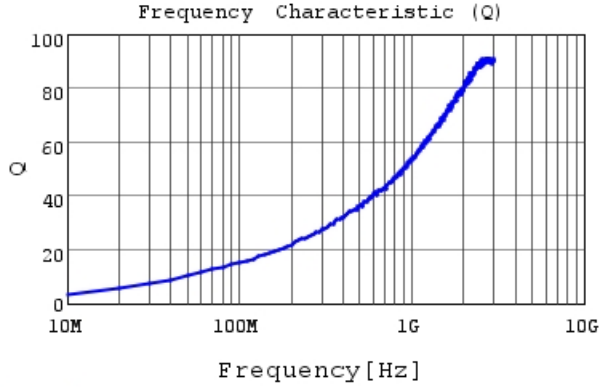
LQG15WH2N1C02 Q
