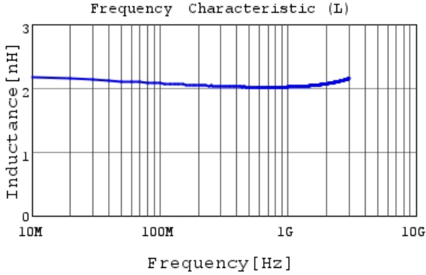
LQG15WH2N1C02 L
