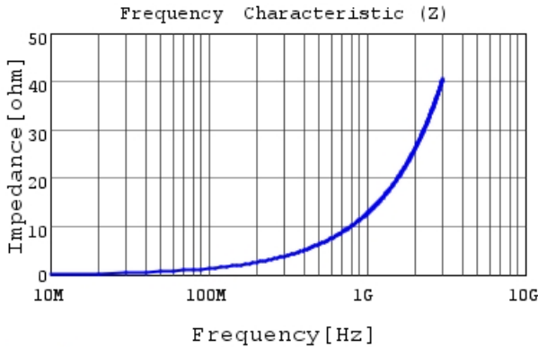
LQG15WH2N1C02 |Z|
