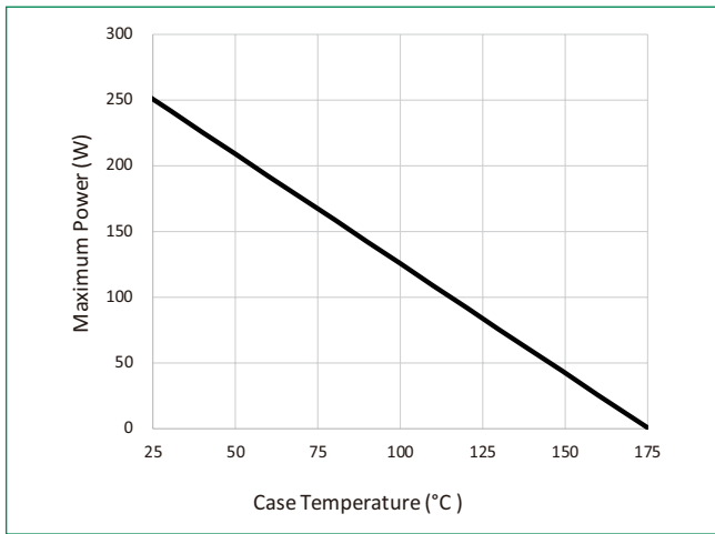
Figure 3: Power Derating (Per Leg)
