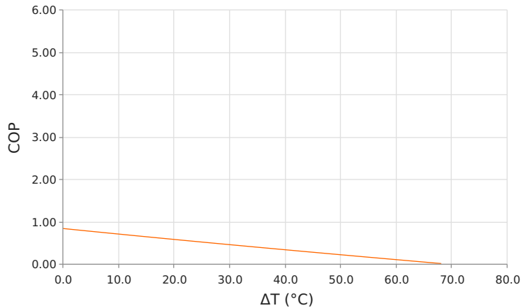
Coefficient of Performance (COP = Qc/Pin) Thot = 85 °C | Current = 1.0 Amps
