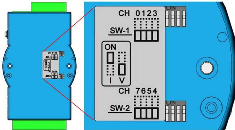
ADAM-6017-D current/voltage input range switch setting
