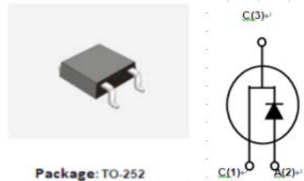
Package: TO-252
