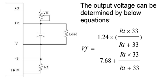
Figure1 The schematic of output voltage adjusted by using external resistor and/or variable resistor.
