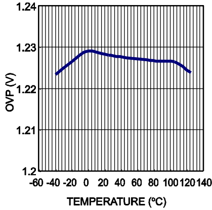
OVP Voltage vs. Temperature
