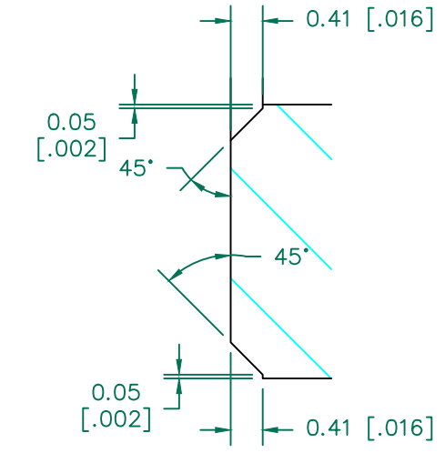
DETAIL "A" CHAMFER SCALE=4:1 (TYPICAL)
