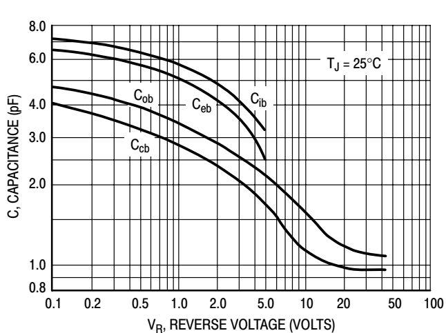
Figure 11. Capacitance
