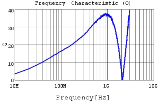
LQG15WH43NJ02 Q
