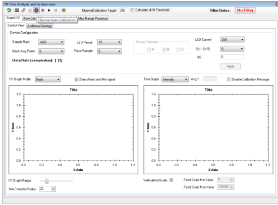
Figure 6. Running the Channel Auto Calibration
