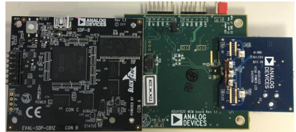
Figure 9. Connecting the ADUX1020-EVALZ-LED Daughterboard
