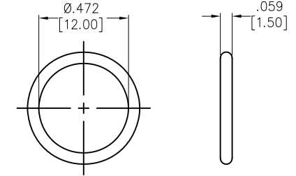
O-RING
