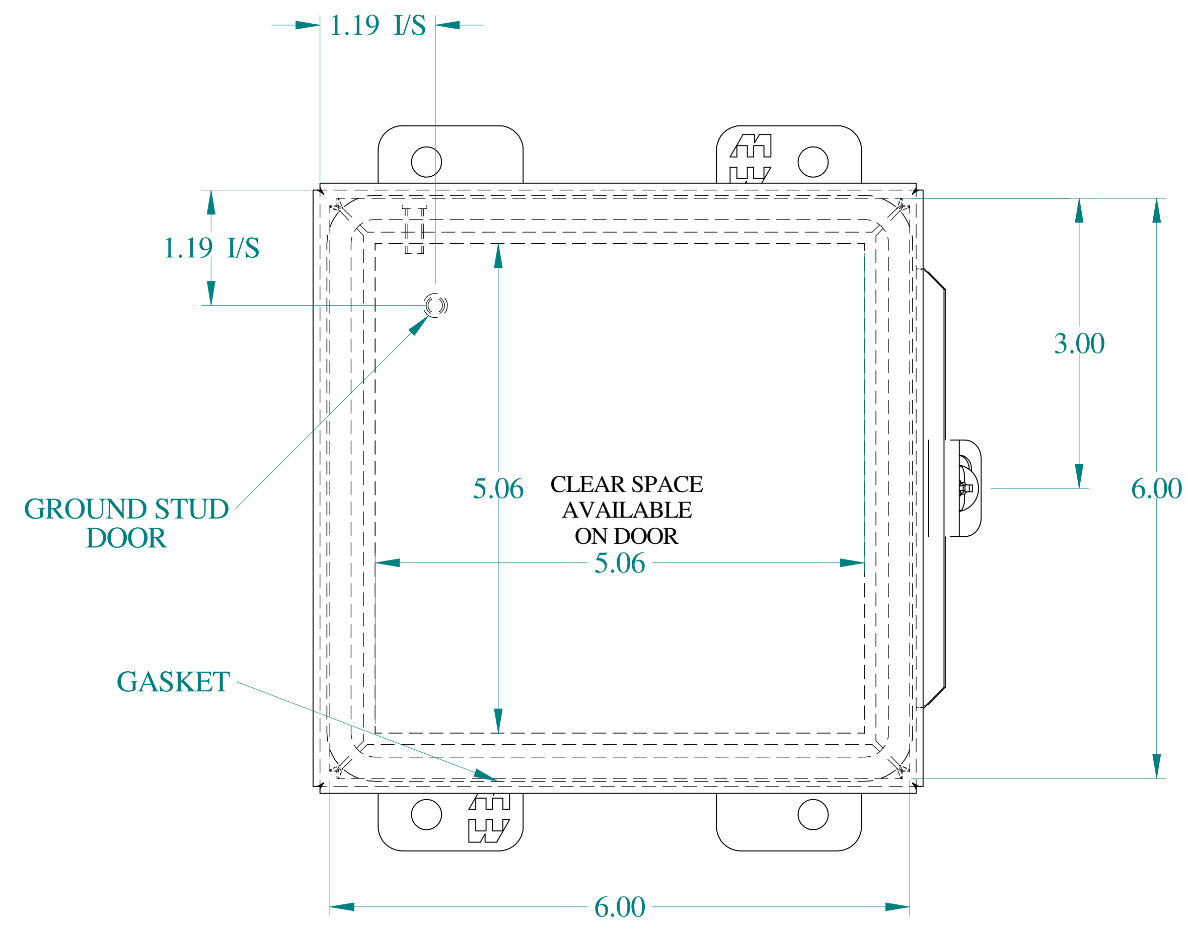
FRONT VIEW
