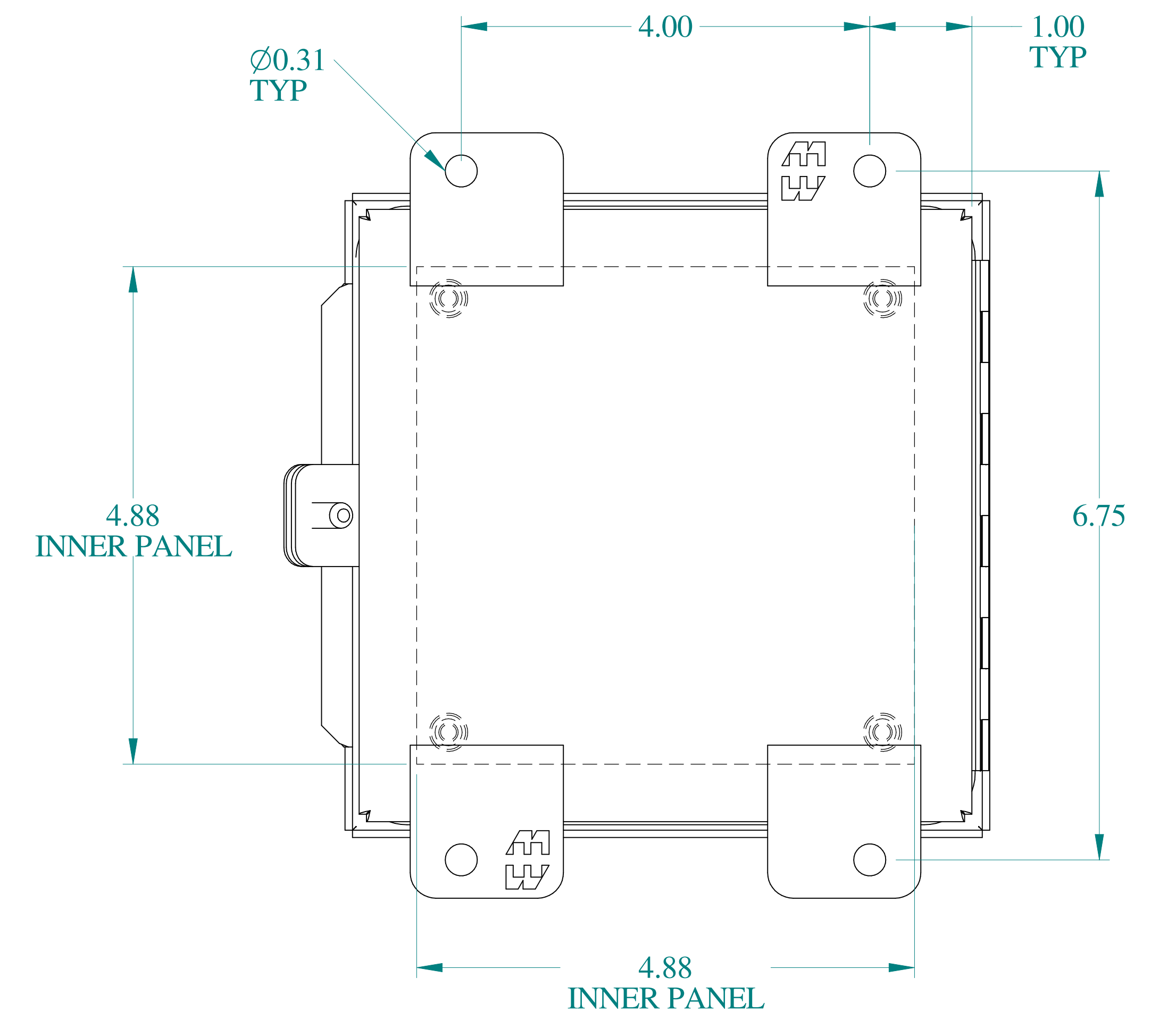
BACK VIEW
