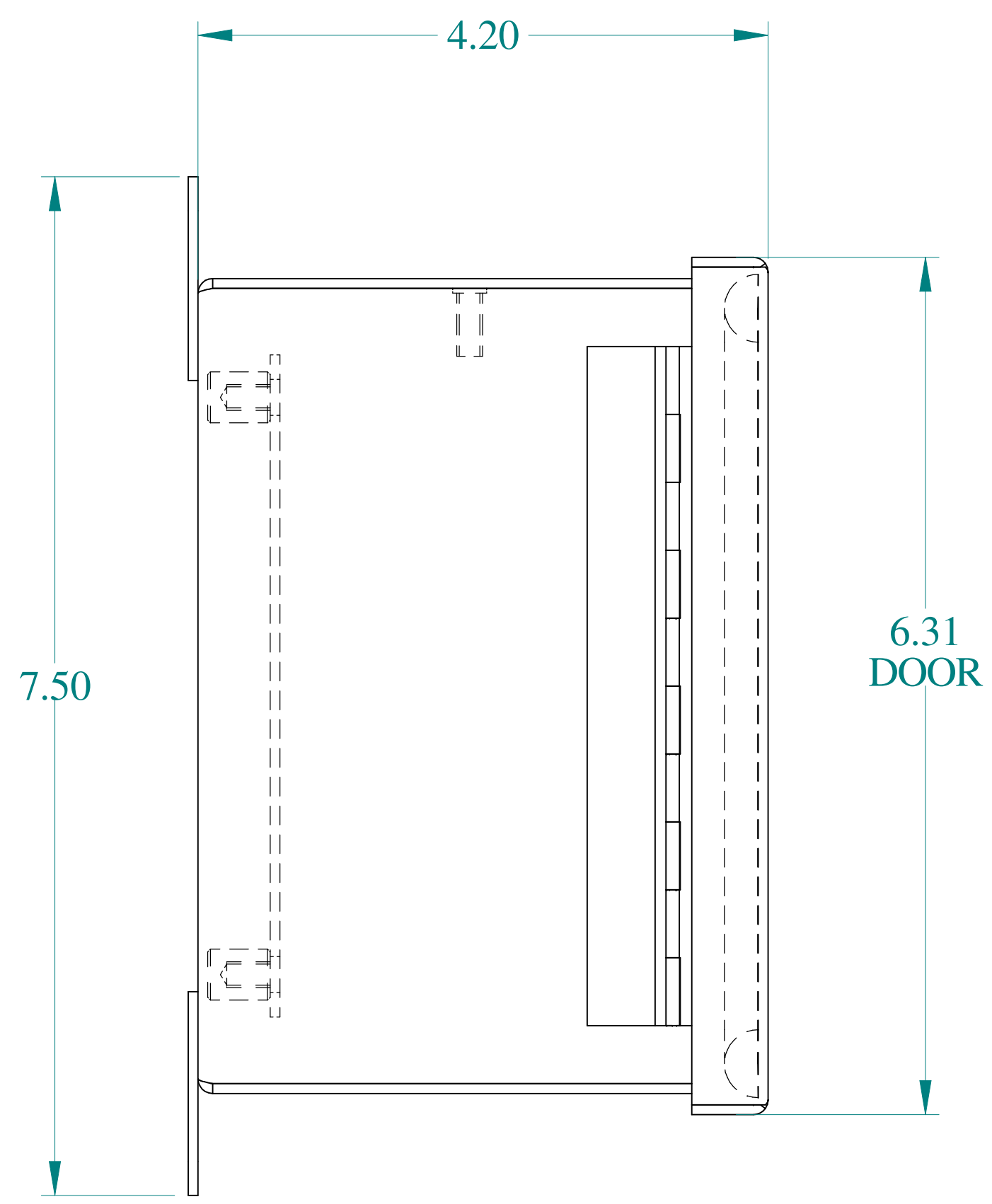
SIDE VIEW
