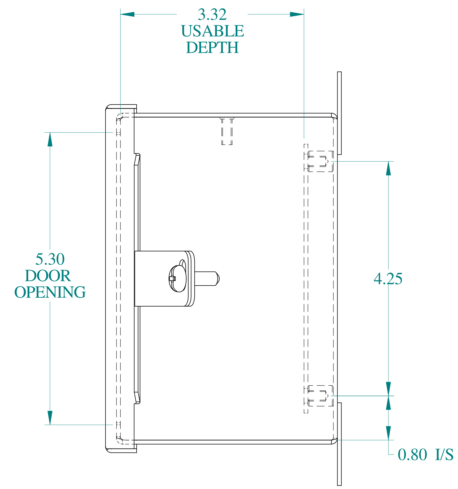
SIDE VIEW
