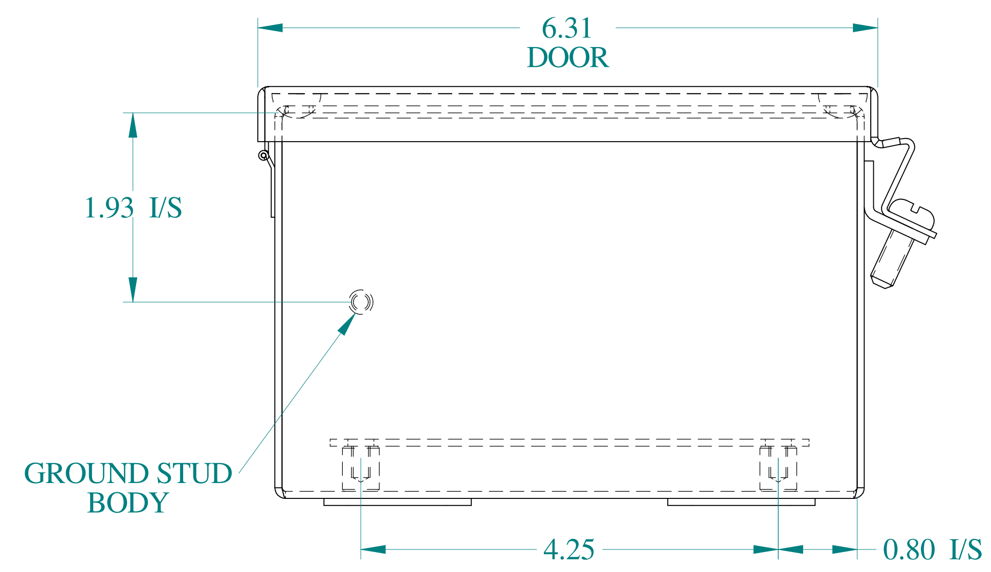
BOTTOM VIEW
