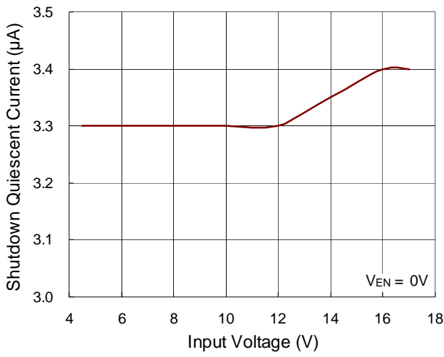
Shutdown Quiescent Current vs. Input Voltage
