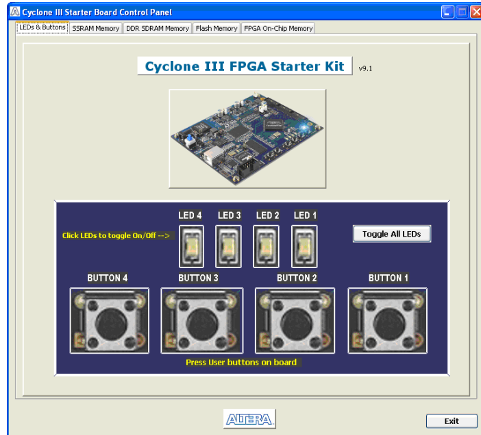
Figure 3–2. Control Panel Window for LEDs and Buttons
