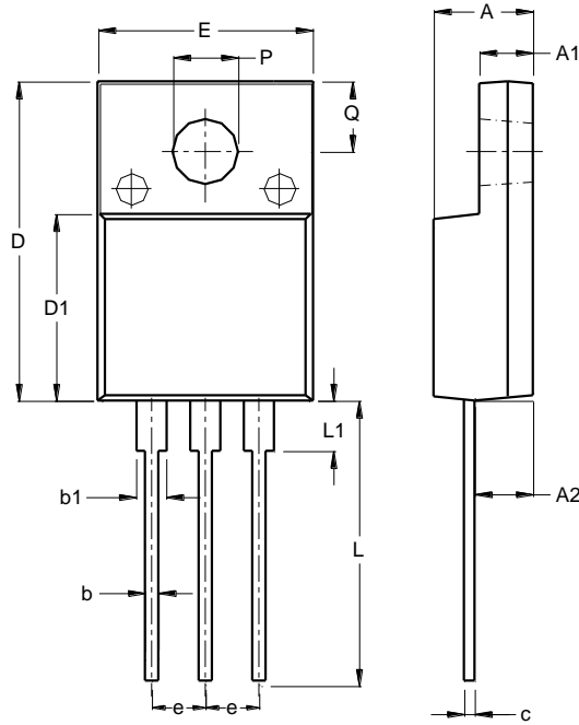
ITO220AB (Type WX2)
