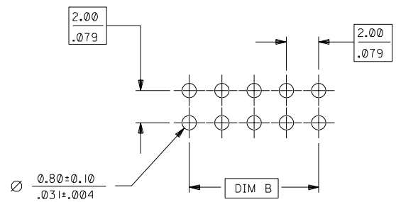
RECOMMENDED PCB PATTERN (SCALE 5:1)
