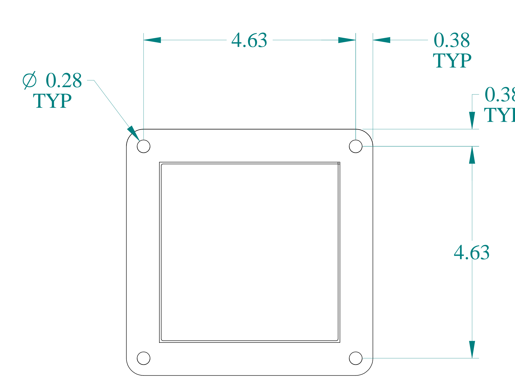
SIDE VIEW
