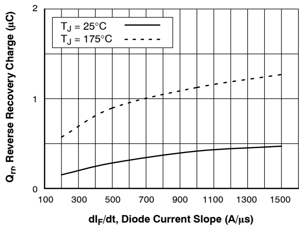
Figure 18. Stored Charge
