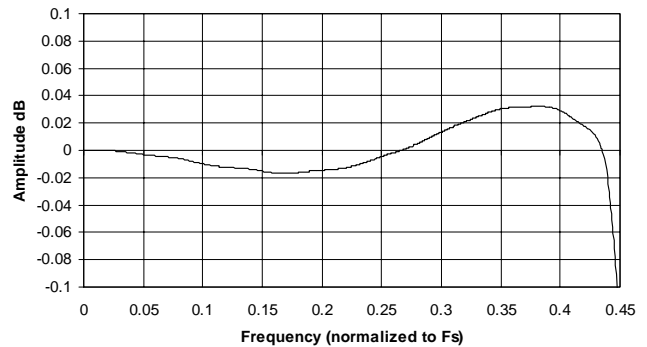
Figure 14. Double-speed Frequency Response
