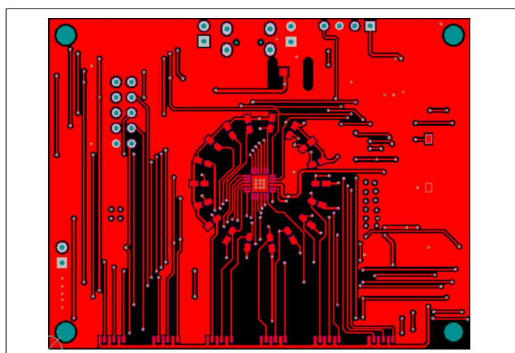
Figure 5: Board PCB Layout - Top Layer
