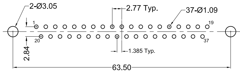
Recommended PCB Layout (Top View)
