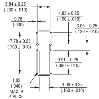
Improved Design
