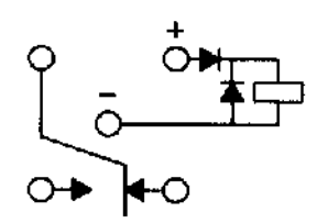
TERMINAL VIEW
