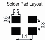
Solder Pad Layout
