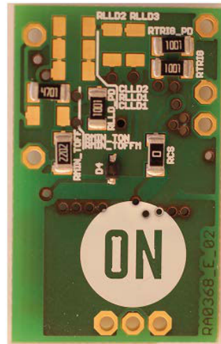
Figure 1. NCP4305 Evaluation Board
