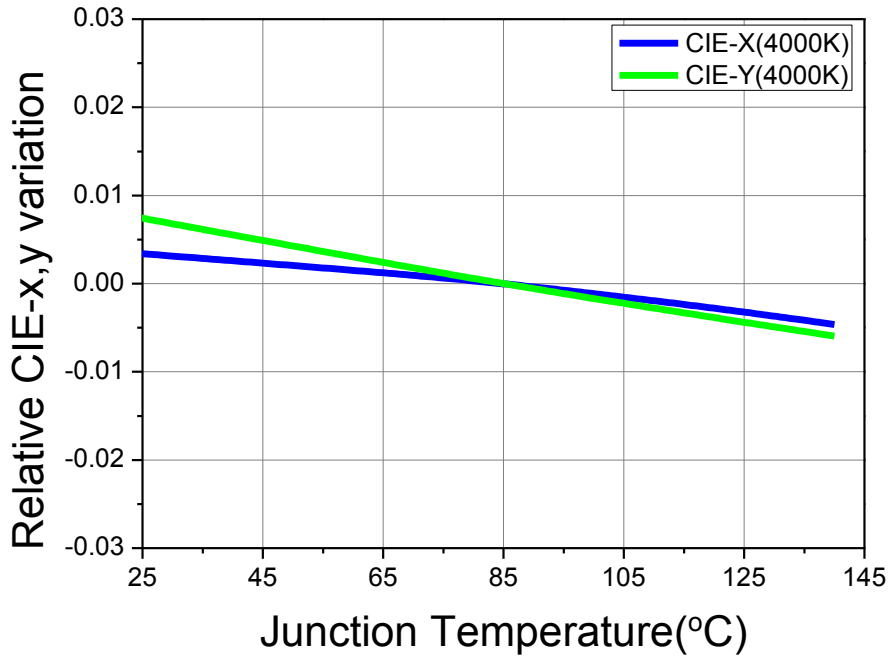
Fig 11. Junction Temperature vs. CIE x,y Shift, I_F=1.1A (CRI90, 4000K)
