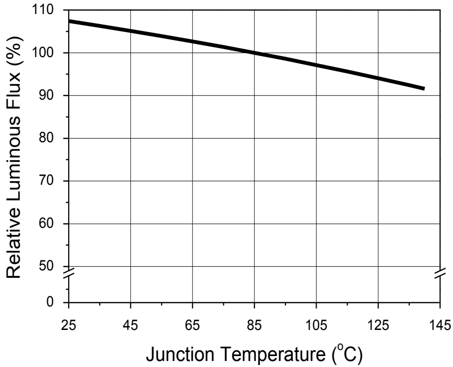
Fig 6. Junction Temperature vs. Relative Luminous Flux, I_F=1.1A
