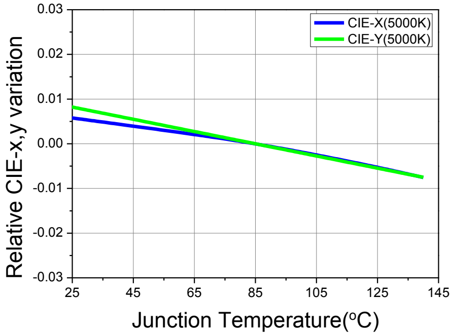
Fig 8. Junction Temperature vs. CIE x,y Shift, I_F=1.1A (CRI80, 5000K)
