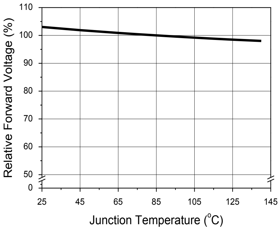
Fig 7. Junction Temperature vs. Forward Voltage, I_F=1.1A
