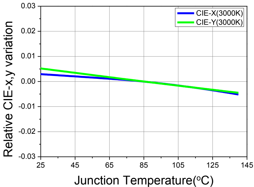
Fig 12. Junction Temperature vs. CIE x,y Shift, I_F=1.1A (CRI90, 3000K)
