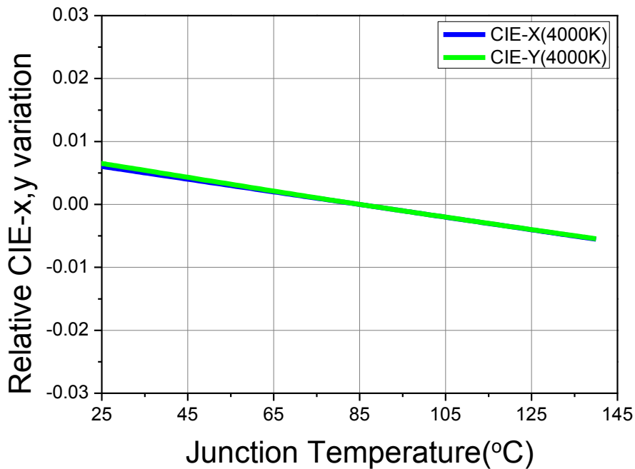
Fig 9. Junction Temperature vs. CIE x,y Shift, I_F=1.1A (CRI80, 4000K)
