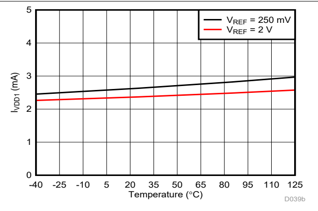
Figure 6-30. High-Side Supply Current vs Temperature
