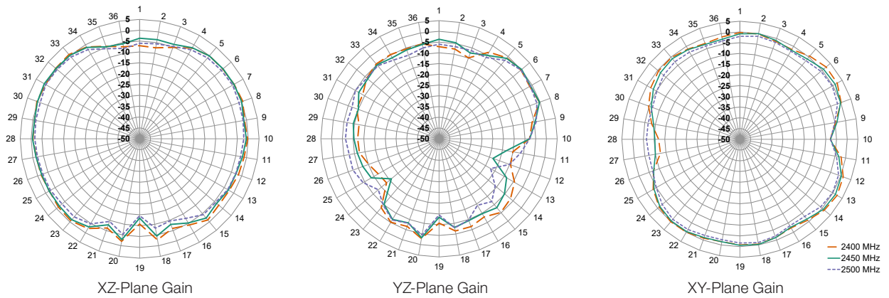
Figure 16. Radiation Patterns for MON-L on Edge of Ground Plane, Bent at 90 Degrees
