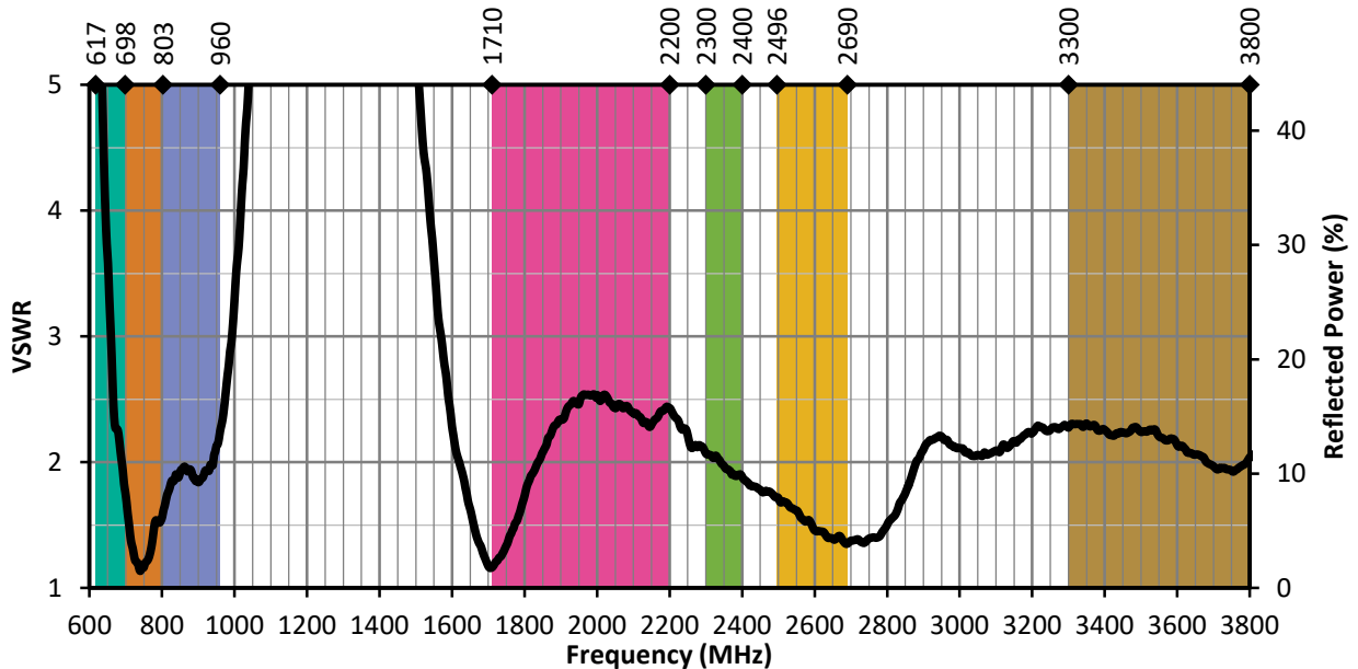
Figure 11. MON-L VSWR, Edge-Bent, with Frequency Band Highlights
