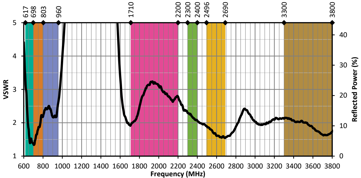
Figure 4. MON-L VSWR, Edge-Straight, with Frequency Band Highlights
