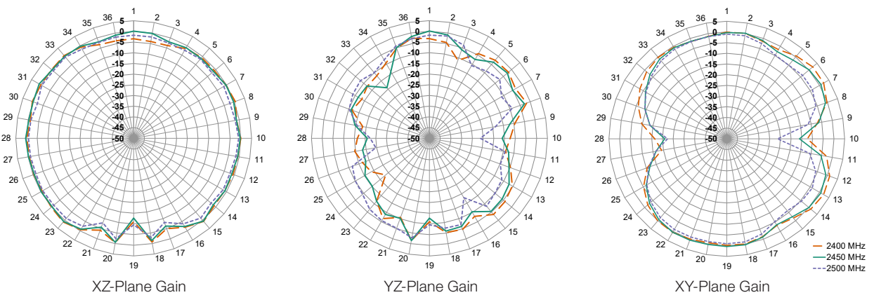
Figure 9. Radiation Patterns for MON-L on Edge of Ground Plane, Straight
