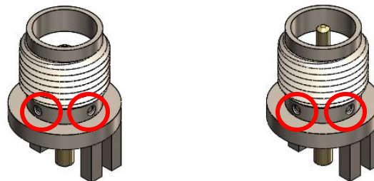
Figure 2: CONSMA003.031 and CONREVSMA003.031 with insulation retention dimples
