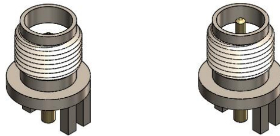
Figure 1: CONSMA003.031 and CONREVSMA003.031 without insulation retention dimples
