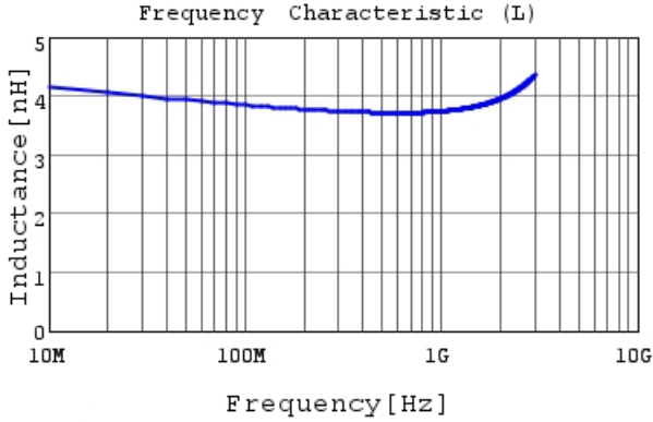
LQG15WH3N8S02 L
