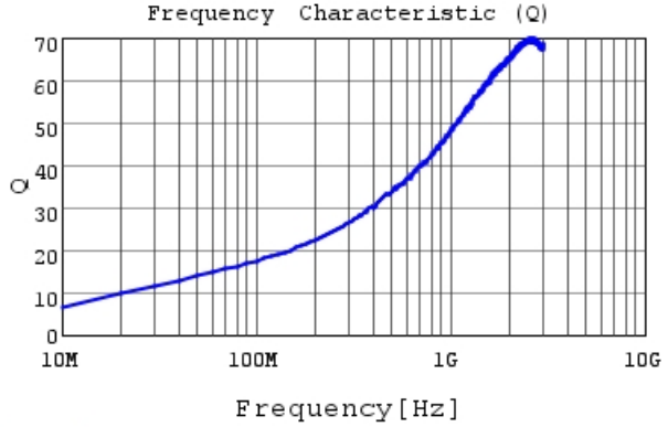
LQG15WH3N8S02 Q
