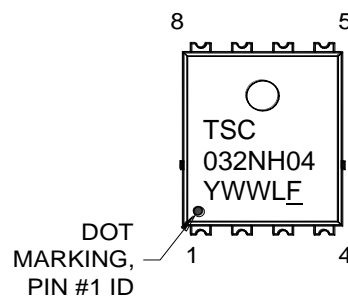
MARKING DIAGRAM
