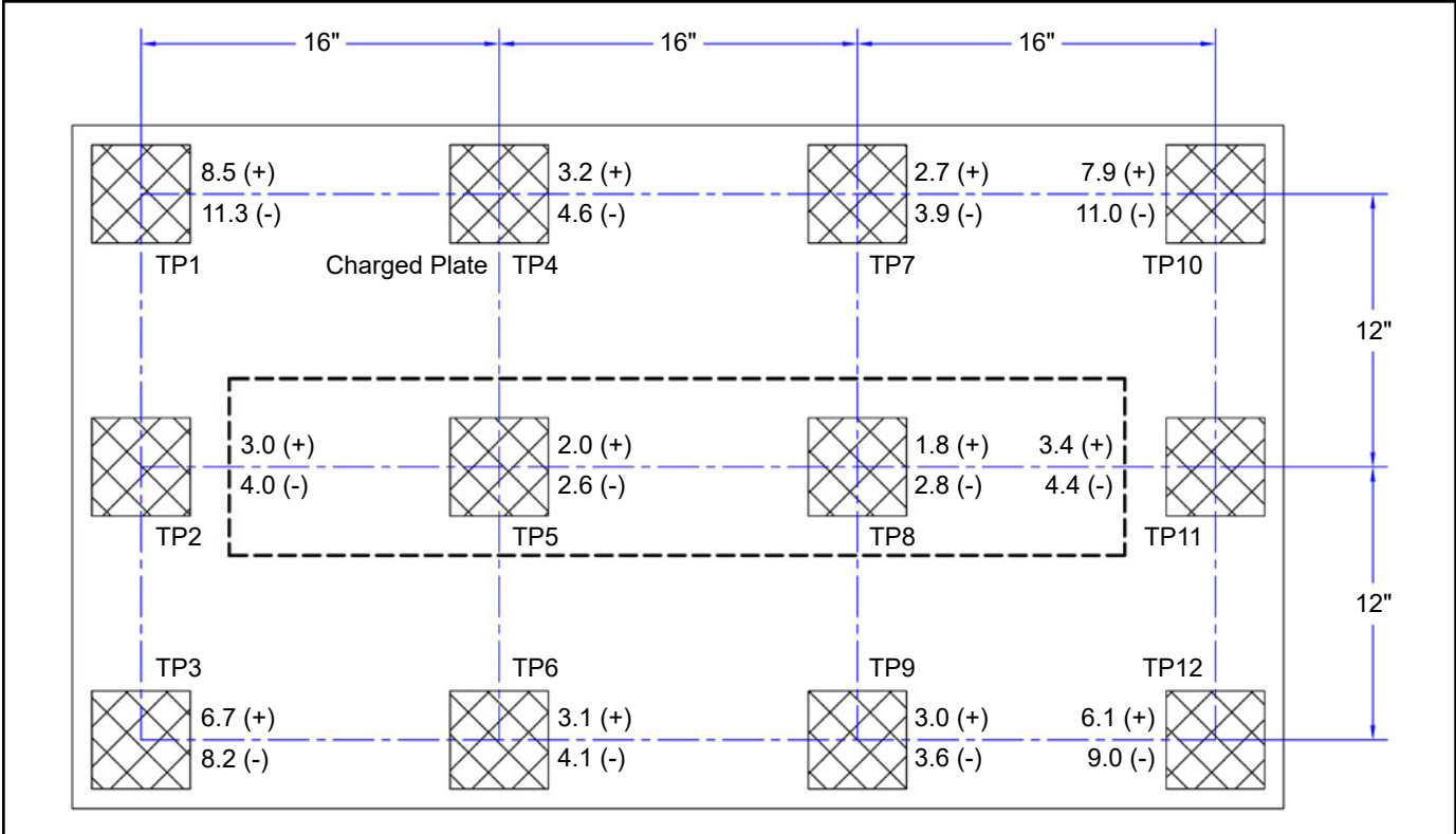
Figure 10. 50665 Neutralization (Discharge) Times at 120VAC, 60Hz input
