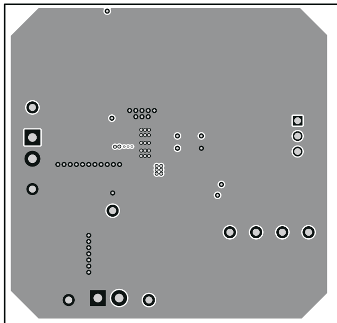
Figure 5-3. Internal Layer 1
