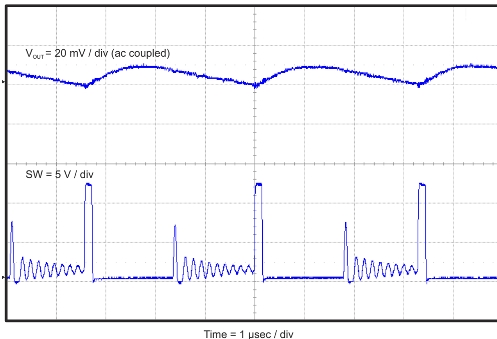
Figure 4-8. TPS54339EEVM-056 Output Voltage Ripple ( I_{OUT} = 150 \text{ mA} )
