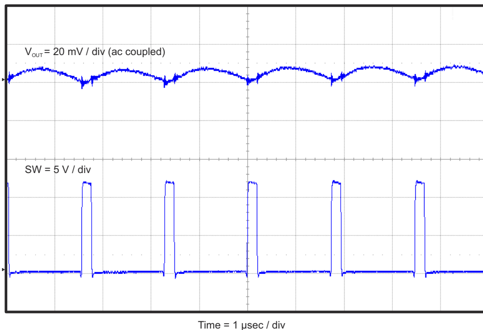
Figure 4-7. TPS54339EEVM-056 Output Voltage Ripple ( I_{OUT} = 3 \text{ A} )
